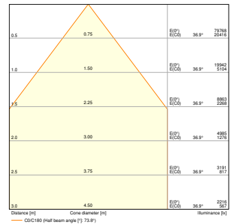
HB P 200W 865 110DEG IP66 PS - REFRACTOR
