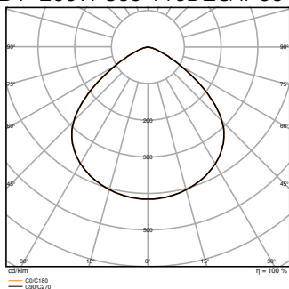
HB P 200W 865 110DEG IP66 PS set to 173W
