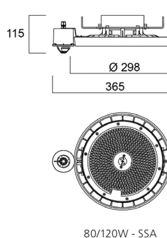
80/120W - SSA
